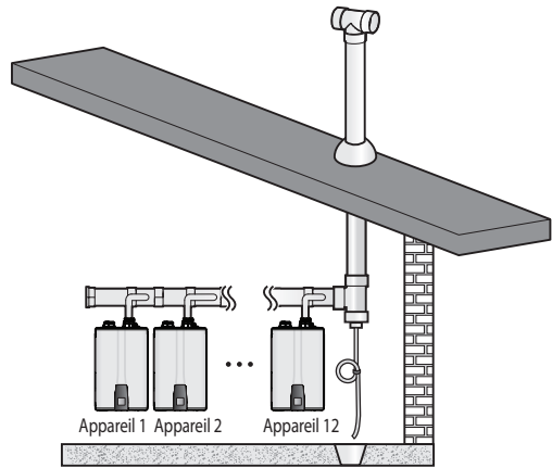
[Ventilation indirecte]
