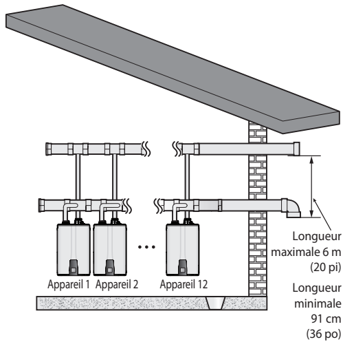
[Ventilation directe]
