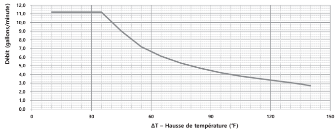
[NPE-240A2]
