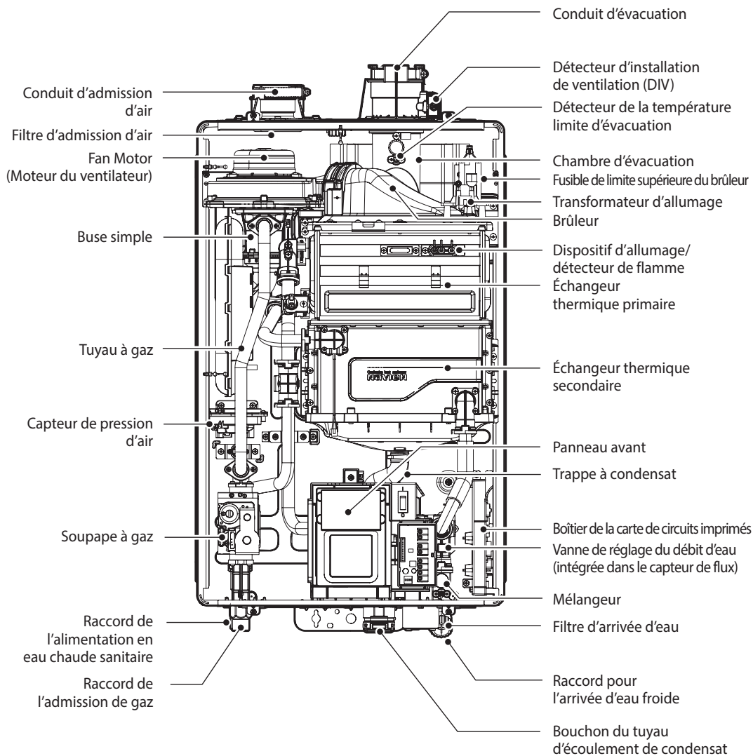
[NPE-150S2]
