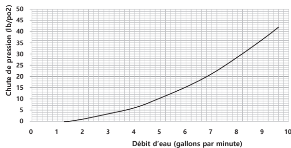
[NPE-150S2]
