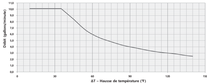
[NPE-210A2]
