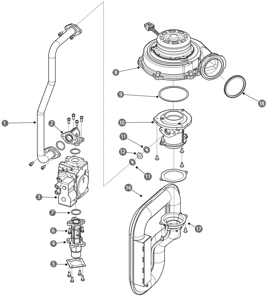
[NPE-150S2]
